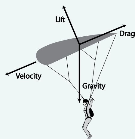
Figure 6-1. The forces acting upon a canopy in flight.
